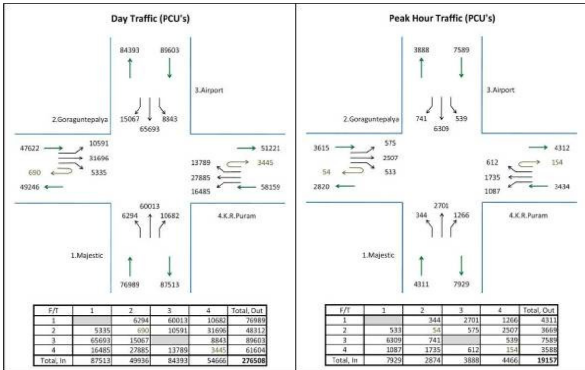
Figure 5-9 Hebbal Junction - Peak hour and daily traffic
