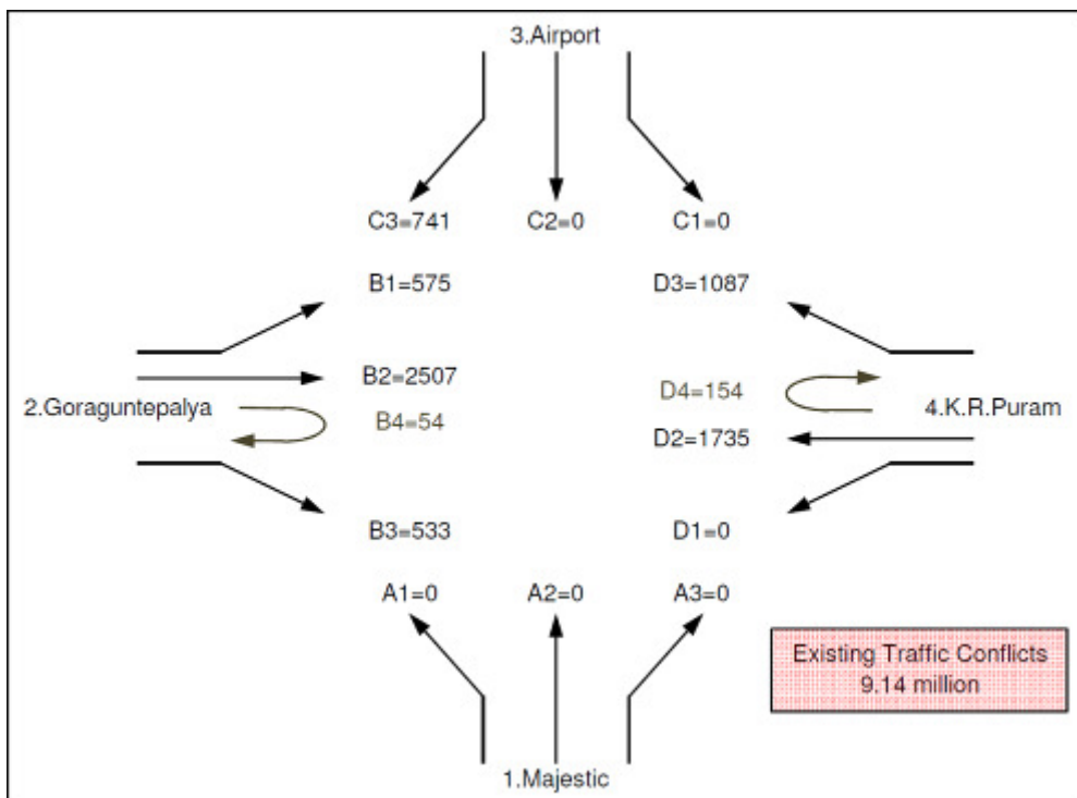
Figure 5-41 Hebbal Junction - Traffic Conflicts
