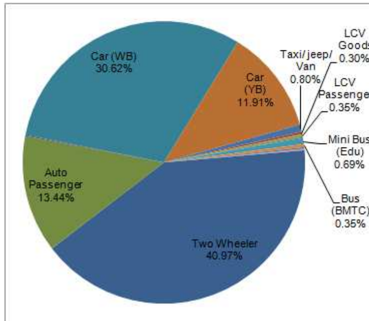
Figure 5-20 Composition of Traffic at Basaveshwara Circle
