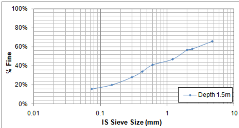
Figure 6-28 Grain Size Analysis for BH-13
