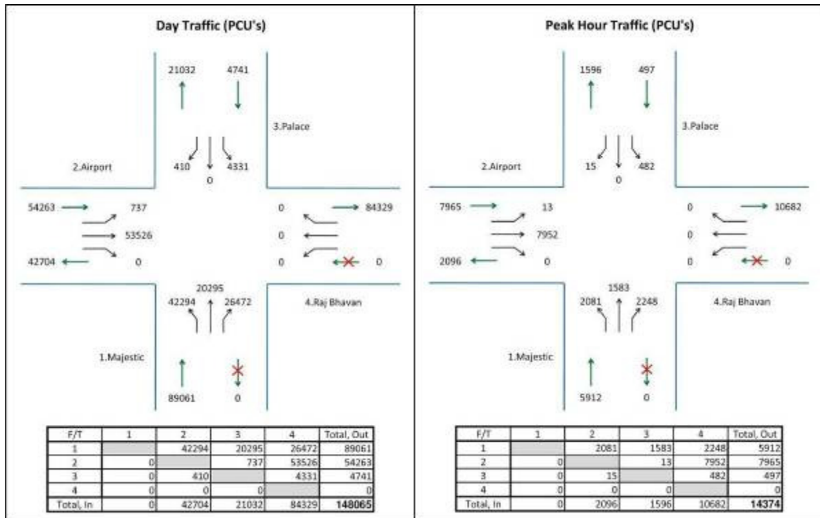
Figure 5-3 Highgrounds Junction - Peak hour and daily traffic
